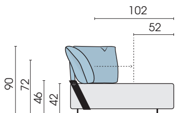
Side view (type 11M/21M/57M)
