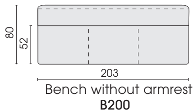
Front view type B200
