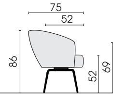
Side view, armchair
